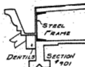
No. 901 Mesker Marquise. A very attractive moderate priced design. Recommended for store fronts especially where transom bars are low.
